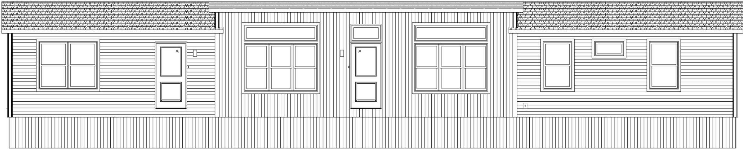
1 MINI HOME - FRONT ELEVATION 3/16" = 1'-0"
